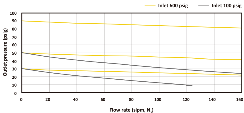
W1500 HF Flow curve
